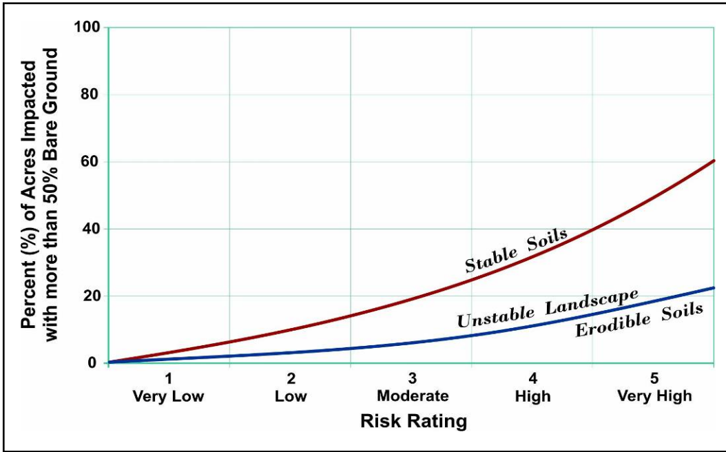
Figure 4-7. Surface erosion risk based on percent of acres impacted with more than 50% bare ground by soil type.
